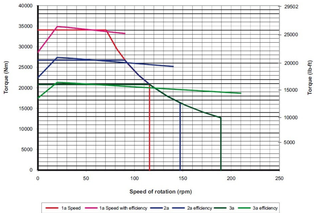
HTD250 TOP DRIVE PERFORMANCE
